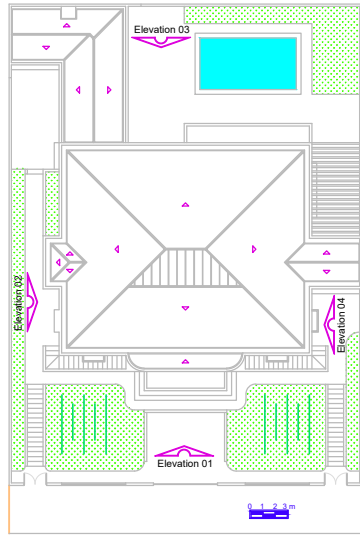
Roof Plan
