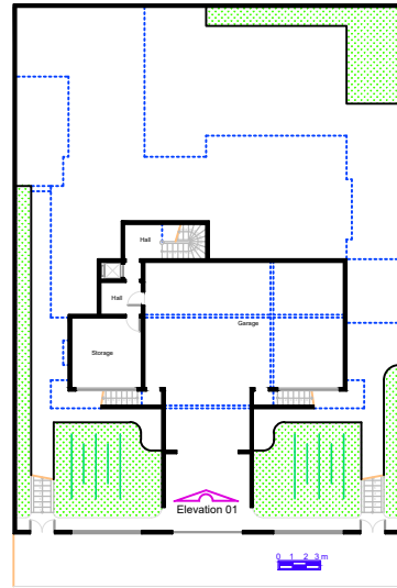
Lower Floor Plan A = 141,06 m 2
