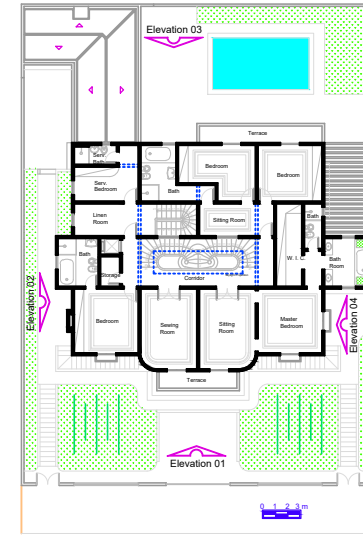
Second Floor Plan A = 222,00 m 2
